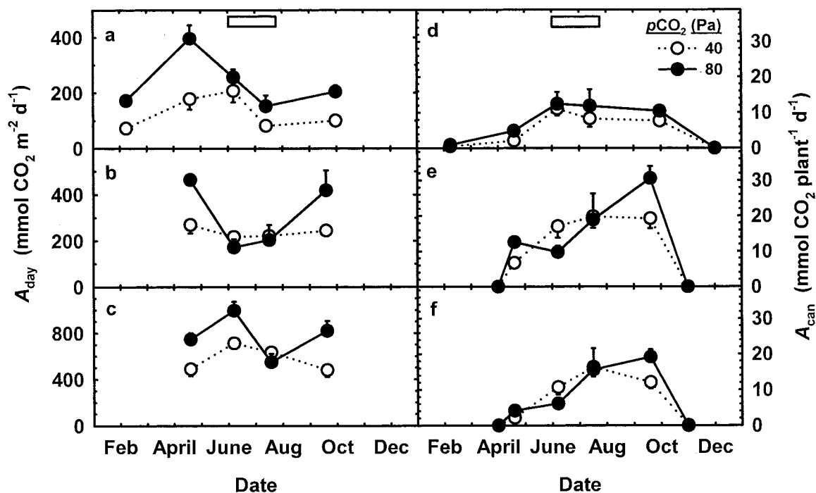
Figure 7. Scaling of leaf photosynthesis in time and space. Estimates of total daily CO 2 fixation by individual leaves ( A_{\text{day}} ; millimoles CO 2 per meter squared per day) are shown in a through c, and gross daily CO 2 fixation by each plant ( A_{\text{can}} ; millimoles CO 2 per plant per day) are shown in d through f. Zero values were set for A_{\text{can}} during the leafless period in deciduous species (e and f) and the dark period in the evergreen (d). Remaining values are the mean \pm SEM for coastal redwood (a and d), dawn redwood (b and e), and swamp cypress (c and f) grown at a p\text{CO}_2 of 40 or 80 Pa. Bars on the top of graphs indicate the period of continuous light.
