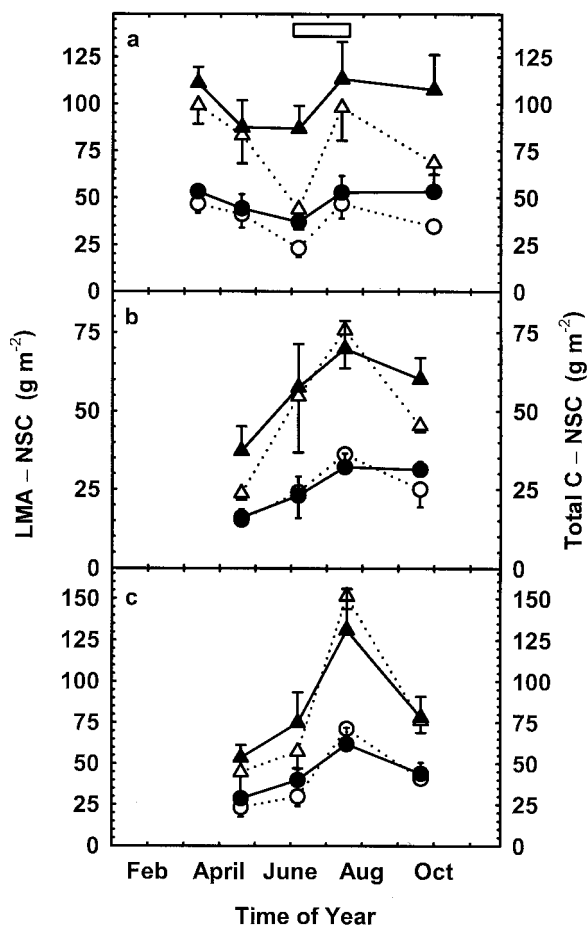
Figure 6. Seasonal changes in LMA ( \Delta and \blacktriangle ) and leaf carbon content ( \circ and \bullet ) in recently expanded leaves, corrected to remove the influence of NSC accumulation. Values are the mean \pm SEM for coastal redwood (a), dawn redwood (b), and swamp cypress (c) grown at a p\text{CO}_2 of 40 Pa ( \Delta and \circ ) or 80 Pa ( \blacktriangle and \bullet ). Bars on the top of graphs indicate the period of continuous light.
