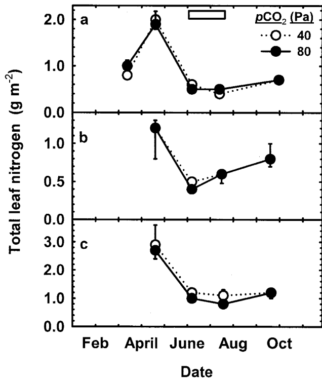
Figure 4. Seasonal changes in the nitrogen content of recently expanded leaves (grams per meter squared) for coastal redwood (a), dawn redwood (b), and swamp cypress (c) grown at a p\text{CO}_2 of 40 or 80 Pa. Values are the mean \pm SEM for four replicate growth rooms. Bars on the top of graphs indicate the period of continuous light.
