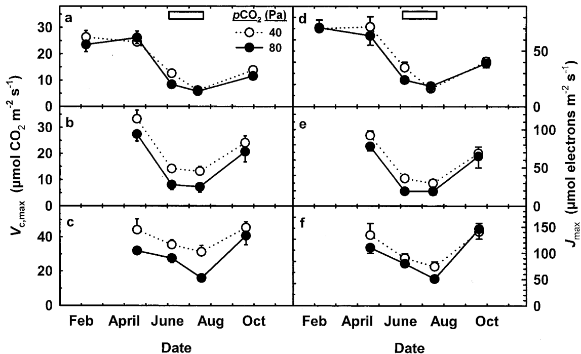
Figure 2. Seasonal changes in V_{c,\text{max}} (micromoles CO 2 per meter squared per second; a–c) and J_{\text{max}} (micromoles electrons CO 2 per meter squared per second; d–f) estimated by analyzing the response of A_{\text{sat}} to C_i in recently expanded leaves. Values are the mean \pm SEM for coastal redwood (a and d), dawn redwood (b and e), and swamp cypress (c and f) grown at a p\text{CO}_2 of 40 or 80 Pa. Bars on the top of graphs indicate the period of continuous light.
