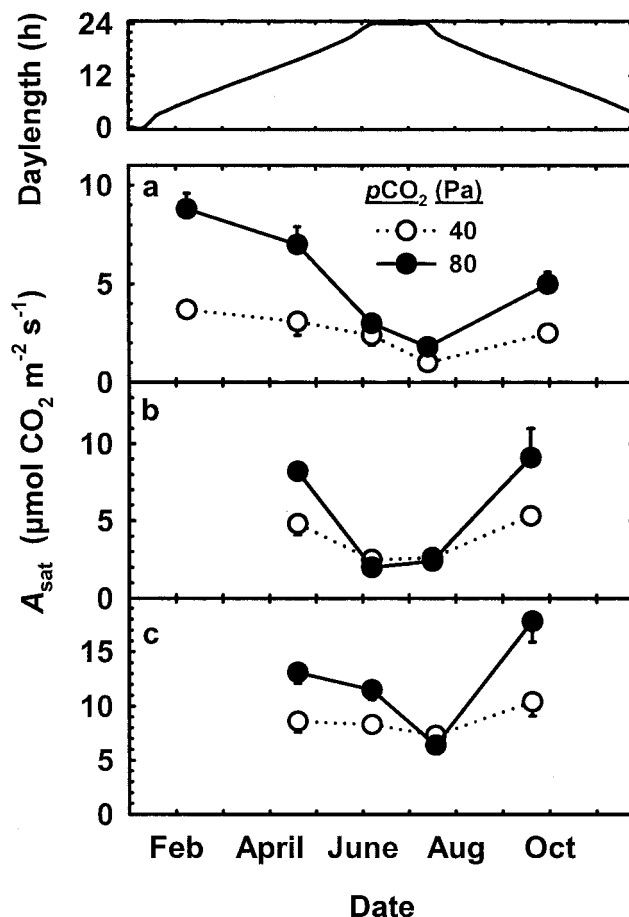
Figure 1. Seasonal changes in daylength (h) and A_{\text{sat}} (micromoles \text{CO}_2 per meter squared per second) for coastal redwood (a), dawn redwood (b), and swamp cypress (c), all grown and measured at a p\text{CO}_2 of 40 or 80 Pa. Measurements were made on recently expanded leaves under standardized conditions, with a leaf temperature of 25°C, and values are the mean \pm SEM for four replicate growth rooms.
