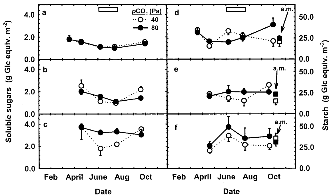
Figure 3. Seasonal changes in the soluble sugar (a–c) and starch (d–f) content of recently expanded leaves (both grams of Glc equivalents per meter squared). Values are the mean \pm SEM for coastal redwood (a and d), dawn redwood (b and e), and swamp cypress (c and f) grown at a p\text{CO}_2 of 40 Pa ( \circ and \square ) or 80 Pa ( \bullet and \blacksquare ). Measurements were made for leaves sampled immediately after the end of the light period, except during the continuous illumination of summer, when samples were taken between 12:00 PM and 3:00 PM ( \circ and \bullet ). Additional samples were taken immediately before the start of the light period in September and are denoted by the square symbols ( \square and \blacksquare ) labeled “a.m.” Soluble sugars are the combined total of Glc, Fru, and Suc contents. Bars on the top of graphs indicate the period of continuous light.
