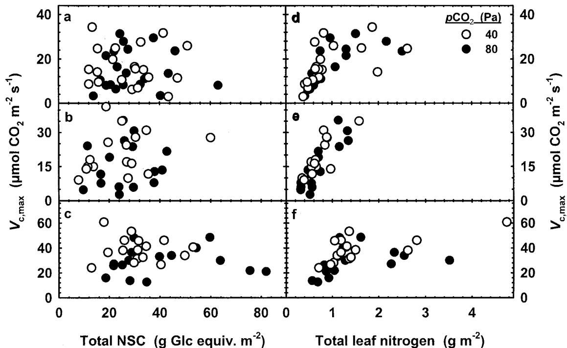
Figure 5. The relationship between V_{c,\text{max}} and leaf NSC and nitrogen contents. Values are individual replicate values from all times of the year in Figures 2A–C, 3, and 4. Relationships between V_{c,\text{max}} and NSC (a–c), and V_{c,\text{max}} and nitrogen contents (d–f) are shown for coastal redwood (a and d), dawn redwood (b and e), and swamp cypress (c and f) grown at a p\text{CO}_2 of 40 or 80 Pa.
